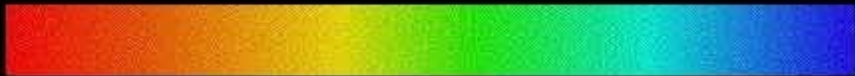
Continuous Spectrum
