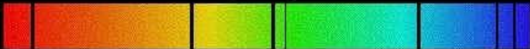
Absorption Spectrum
