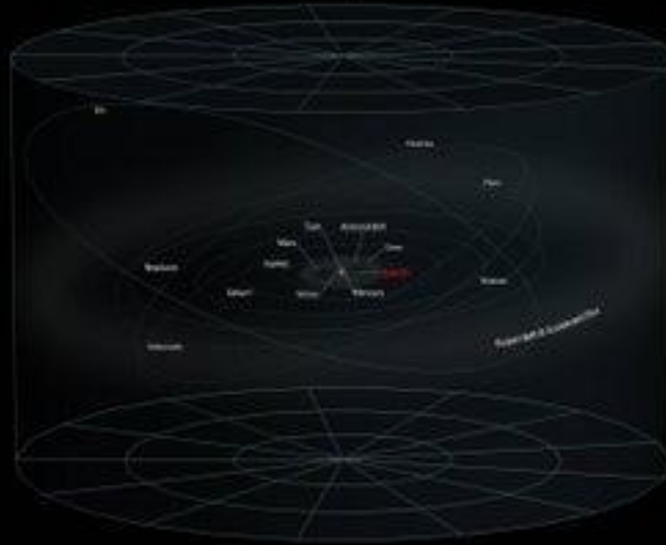
Solar System
