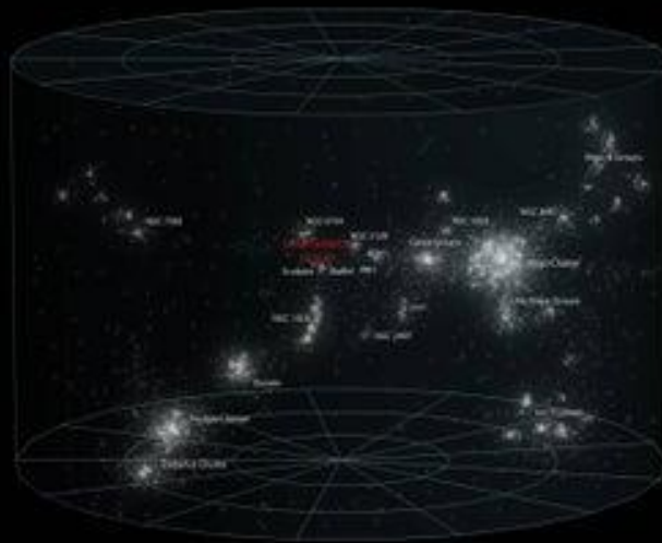
Virgo Supercluster
