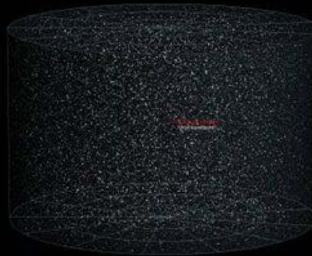
Observable Universe
